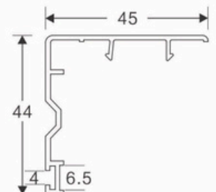
92 SLIDING DOOR SASH COVER CODE: SB-2005
