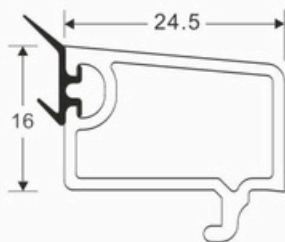
CASEMENT 12MM GLASS BEAD Code: SB-4002
