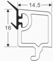
SLIDING 12 MM GLASS BEAD CODE: SB-2001
