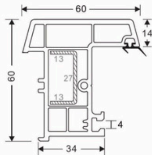
FRENCH MULLION/LAP JOINT CODE : SB-3005
