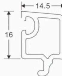
SLIDING 12 MM GLASS BEAD CODE: SB-2001
