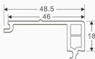
SHUTTER GLAZING BEAD Code: SB-SGB
