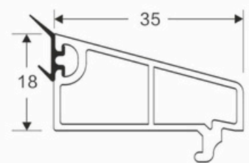
60 CASHMENT Code: SB-3004
