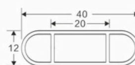
BLIND LOUVER Code: SB-CLP
