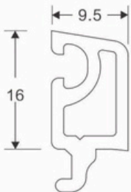
SLIDING 22 MM GLASS BEAD CODE : SB-2002
