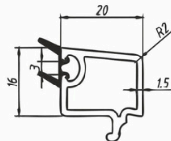
SECTION NAME- SINGLE GLAZING BEAD CODE - 106 WEIGHT - 0.225 KG/MTR STANDARD PACKAGES- 30 Pcs.
