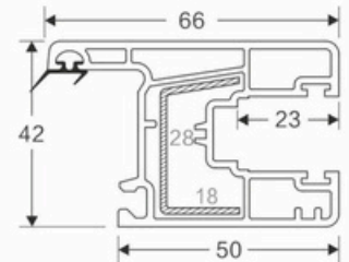
66 SLIDING WINDOW SASH CODE: SB-1004
