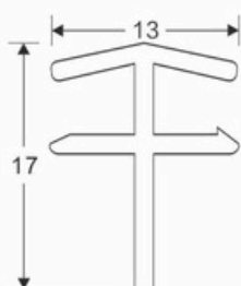
FRAME CONNECTOR Code: SB-F1
