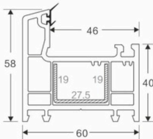
60 CASMENT OUTER FRAME Code: SB-3001
