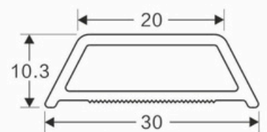
30 MM D. STRIP Code: SB-D1
