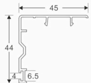
92 SLIDING DOOR SASH COVER CODE: SB-2005
