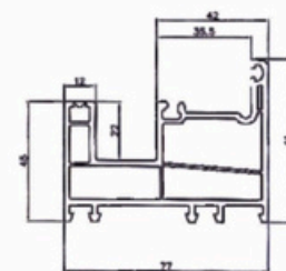
MONORAIL/SLIDING FRAMR CODE: SB-M1
