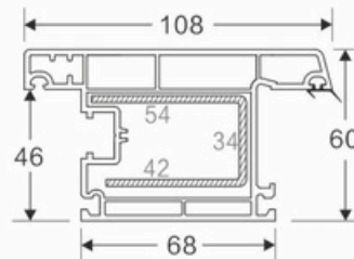
60 OUT WARD DOOR SASH Code: SB-3003
