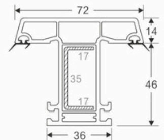
60 CASHMENT Code: SB-3004
