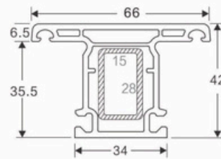
42 SASH SLIDING MULLION 2 CODE: SB-42SM
