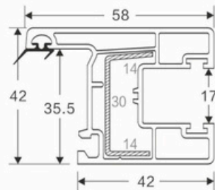
58 SLIDING SASH D CODE: SB-1006
