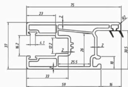
SECTION NAME- SLIDING DOOR SASH CODE - 104 WEIGHT - 1.050 KG/MTR STANDARD PACKAGES- 4 Pcs.
