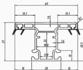
SECTION NAME- INTERLOCK CODE - 107 WEIGHT - 0.18 KG/MTR STANDARD PACKAGES- 30 Pcs.
