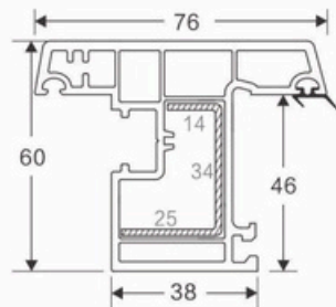
60 OUT WARD WINDOW SASH CODE : SB-3002
