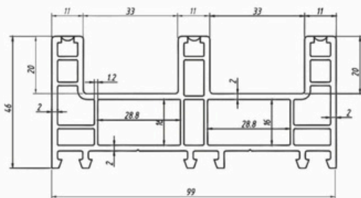
SECTION NAME- 3 TRACK CODE - ECO 102 WEIGHT- 1.46 KG/MTR STANDARD PACKAGES- 4 Pcs.
