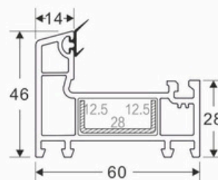
60 OUT WARD DOOR SASH Code: SB-3003
