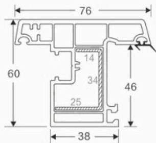
60 OUT WARD WINDOW SASH Code: SB-3002
