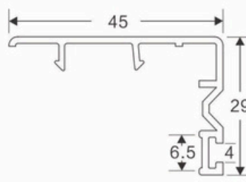
66 SLIDING WINDOW SASH COVER CODE: SB-2004
