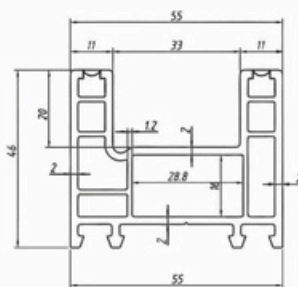
SECTION NAME- 2 TRACK CODE - 101 WEIGHT - 0.930 KG/MTR STANDARD PACKAGES- 6 Pcs.
