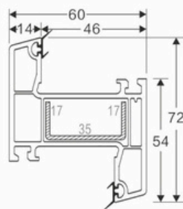
60 SHIFT MULLION Code: SB-3006
