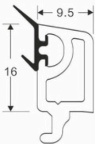
SLIDING 22 MM GLASS BEAD CODE : SB-2002
