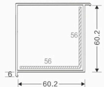
60 RIGHT ANGLE BAY CORNER ADAPTER Code: SB-C90
