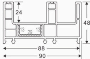
90 SLIDING FRAME 2.5 TRACK CODE : SB-1002
