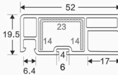
52 SCREEN DOOR SASH CODE: SB-1007
