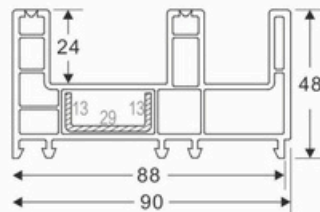
90 SLIDING FRAME 2.5 TRACK CODE: SB-1002
