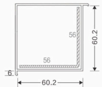
60 RIGHT ANGLE BAY CORNER ADAPTOR CODE : SB-C90
