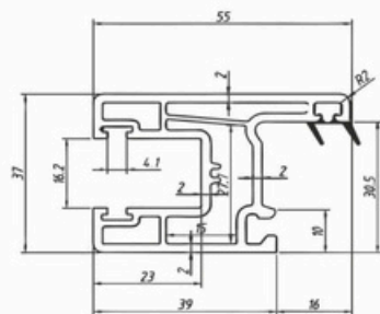
SECTION NAME- SLIDING WINDOW SASH CODE - 103 WEIGHT - 0.840 KG/MTR STANDARD PACKAGES- 8 Pcs.
