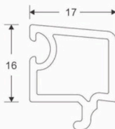
22MM GLAZING BEAD CODE : SB-4003
