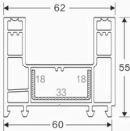
2 TRACK OUTER FRAME CODE : SB-1001
