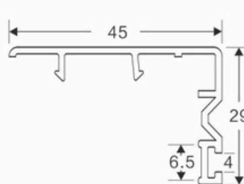
66 SLIDING WINDOW SASH COVER CODE: SB-2004
