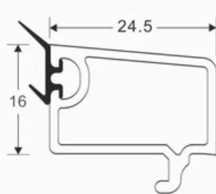
SLIDING SINGLE GALZED BEAD CODE: SB-2003
