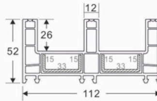
112 SLIDING FRAME-3T CODE: SB-1003
