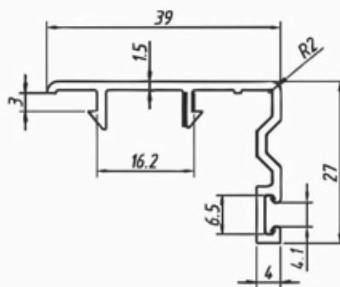
SECTION NAME- SLIDING MULLION CODE - 105 WEIGHT - 0.67 KG/MTR STANDARD PACKAGES- 8 Pcs.
